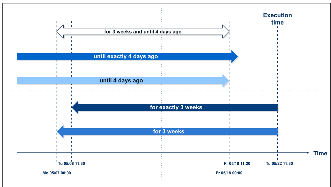
Figure 2.10: Date condition examples
