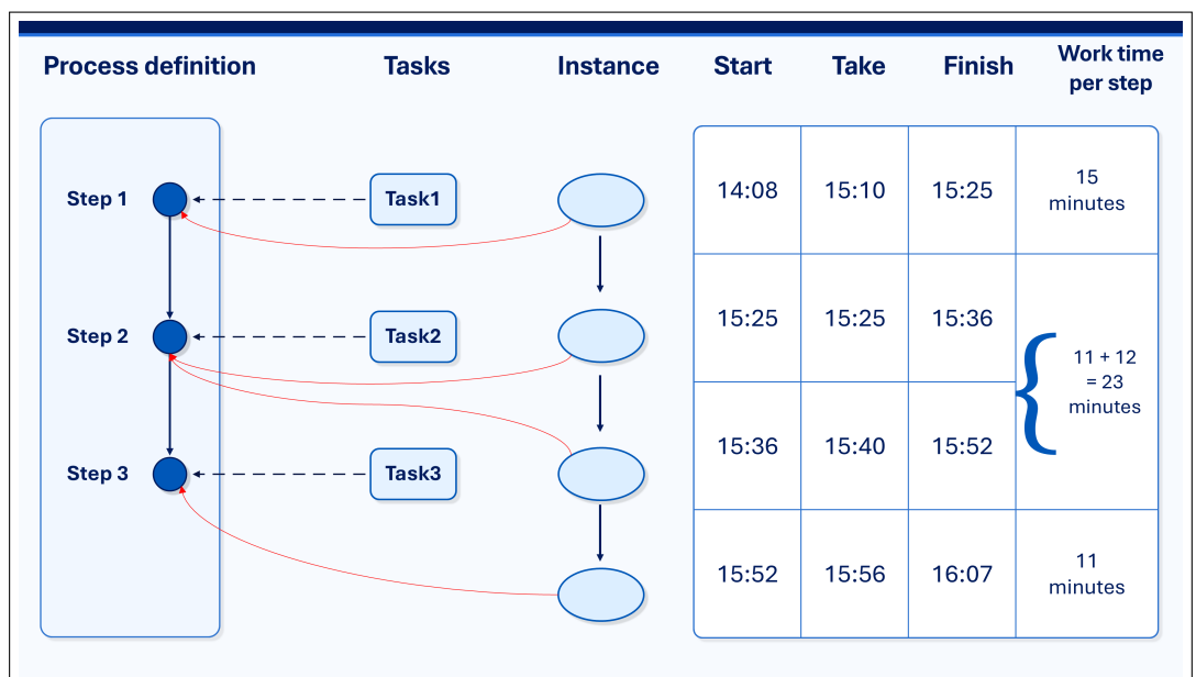
Figure 2.4: Computation of time intervals per step
